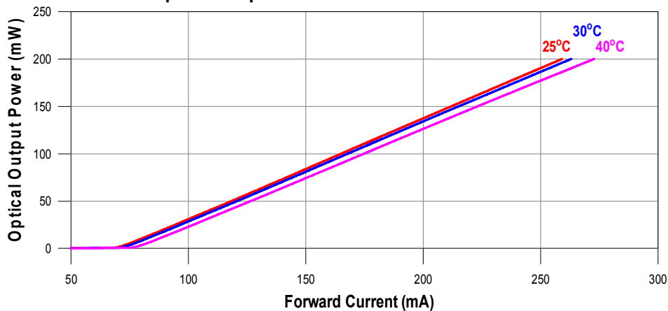
Optical Output Power v.s. Forward Current
