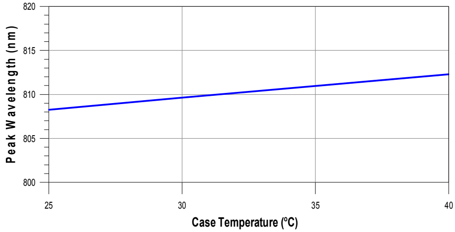
Peak Wavelength v.s. Case Temperature
