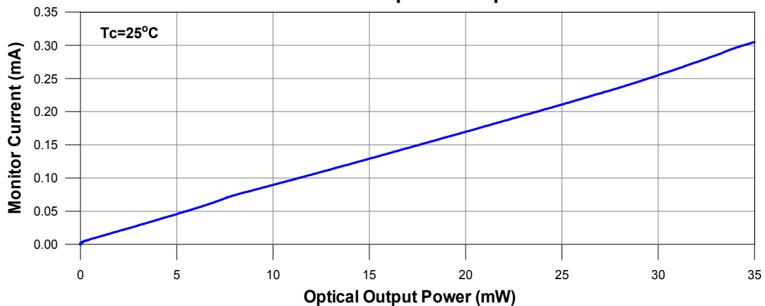
Monitor Current v.s. Optical Output Power
