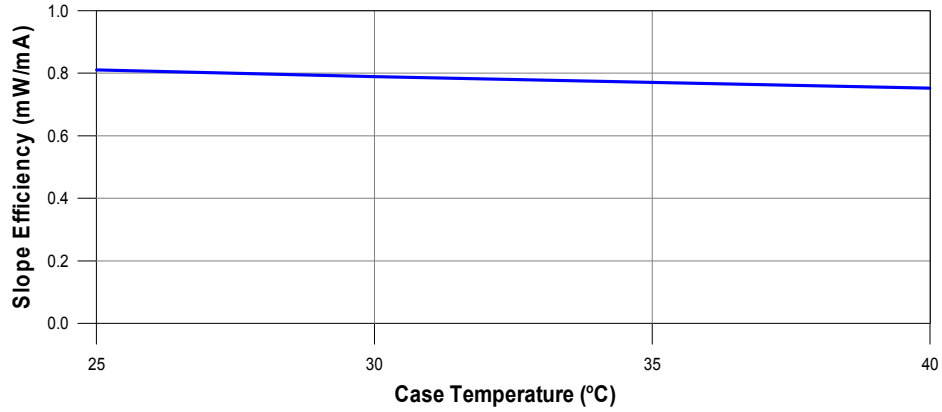
Slope Efficiency v.s. Case Temperature
