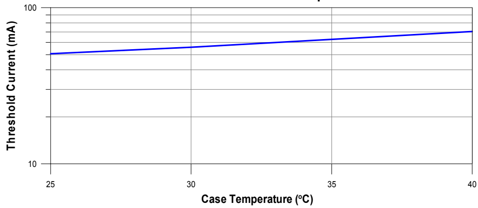
Threshold Current v.s. Case Temperature
