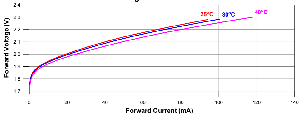
Forward Voltage v.s. Forward Current
