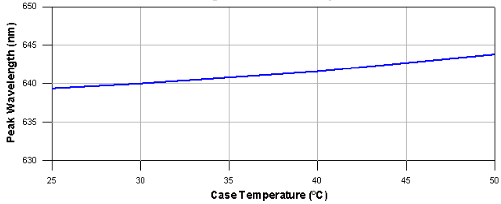
Peak Wavelength v.s. Case Temperature
