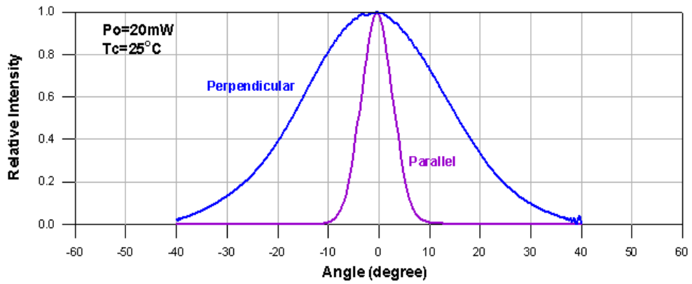
Far-Field Pattern
